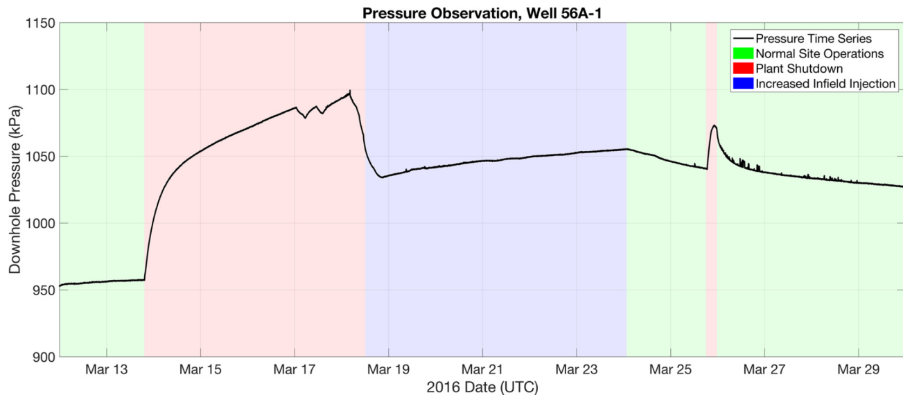
Fig. 2. Pressure changes measured at well 56A-1 during PoroTomo experiment. Colored boxes delineate phases of the PoroTomo experiment. A brief unplanned site shutdown on 2016 March 25 UTC is also delineated.
